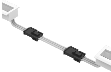
Dry Continuous Connector (20/3 Gauge Wire) (A8-ZUDA-RCD-CC-BFF-DRY-X) X = Specify Length, 3" Default
