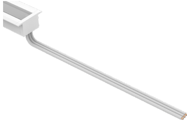
Dry Power Connector (20/3 Gauge Wire) (A8-ZUDA-RCD-PC-BFF-DRY-X) X = Specify Length, 36" Default, 25' Maximum
