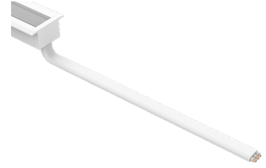
Dry Power Connector with White Jacket (20/3 Gauge Wire) (A8-ZUDA-RCD-PC-BFF-DRY-WH-X) X = Specify Length, 36" Default, 25' Maximum
