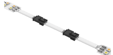
Dry Continuous Connector with White Jacket (20/3 Gauge Wire) (A8-ZOMU-TAPE-CC-DRY-WH-X) X = Specify Length, 3" Default
