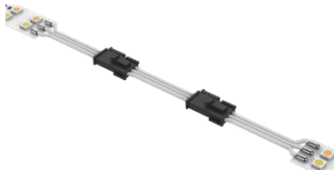
Dry Continuous Connector (20/3 Gauge Wire) (A8-ZOMU-TAPE-CC-DRY-X) X = Specify Length, 3" Default
