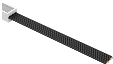
Wet Power Connector (20/5 Gauge Wire) (A8-ZIZA-STN-PC-WET-X) X = Specify Length, 36" Default, 25' Maximum
